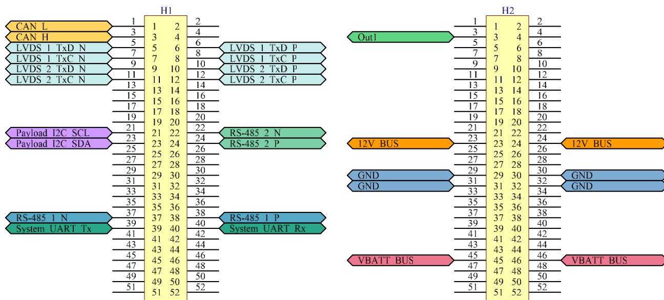
Figure 6 - Pinout of the Stack Connectors
